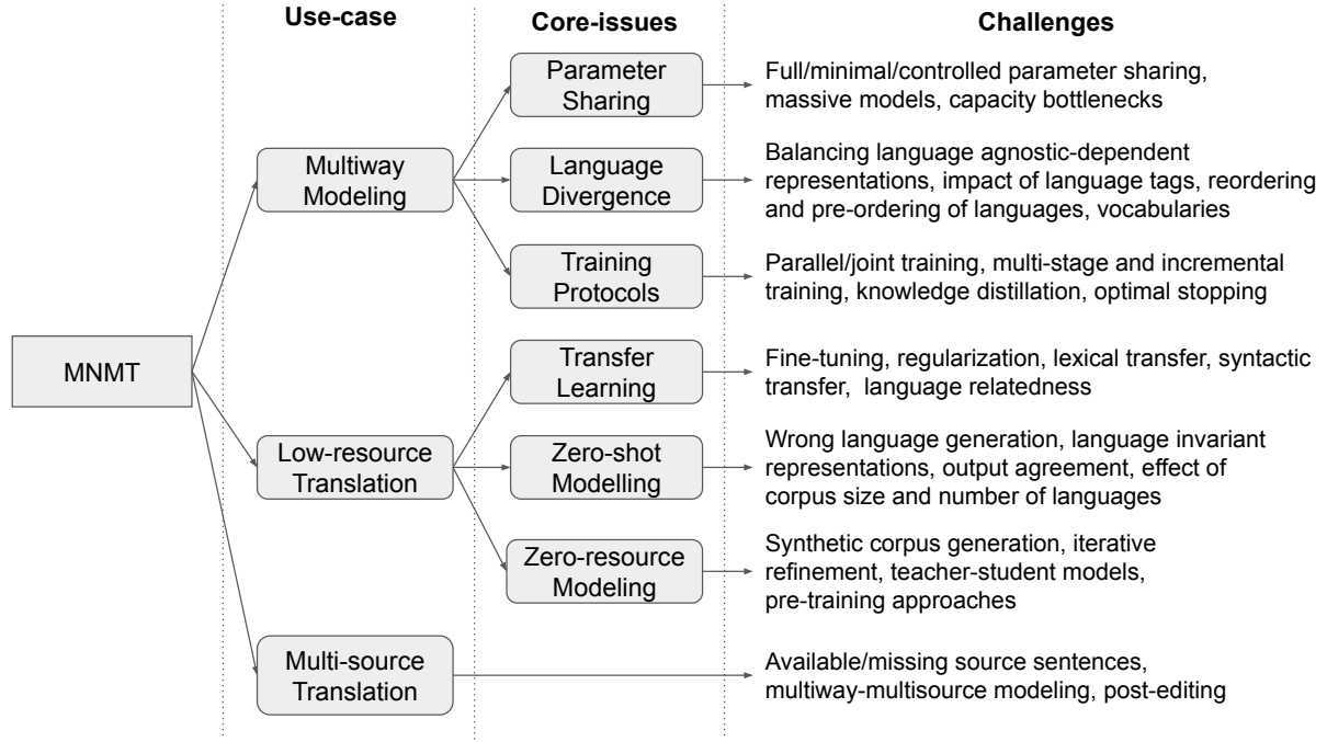
Fig. 1. MNMT research categorized according to use-cases, core-issues and the challenges involved. Note that the focus is on use-cases and an approach for one use-case can be naturally adapted to another use-case and thus can face similar core issues.
